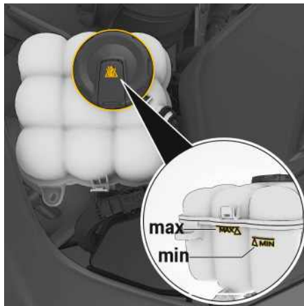
Fig. 58: Coolant reservoir
