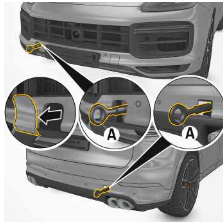
Fig. 208: Towing hook
