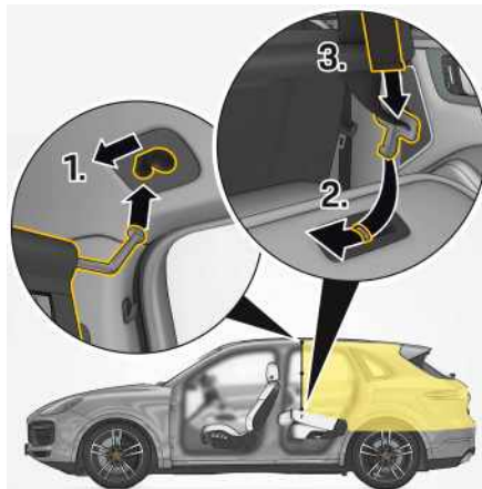
Fig. 115: Installing luggage compartment partition net at the front
