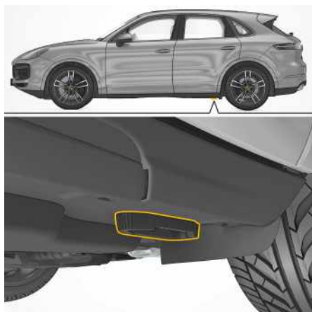
Fig. 85: Jacking point for lifting platform and jack at the rear
