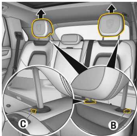
Fig. 181: Removing the headrests from the outer rear seats
