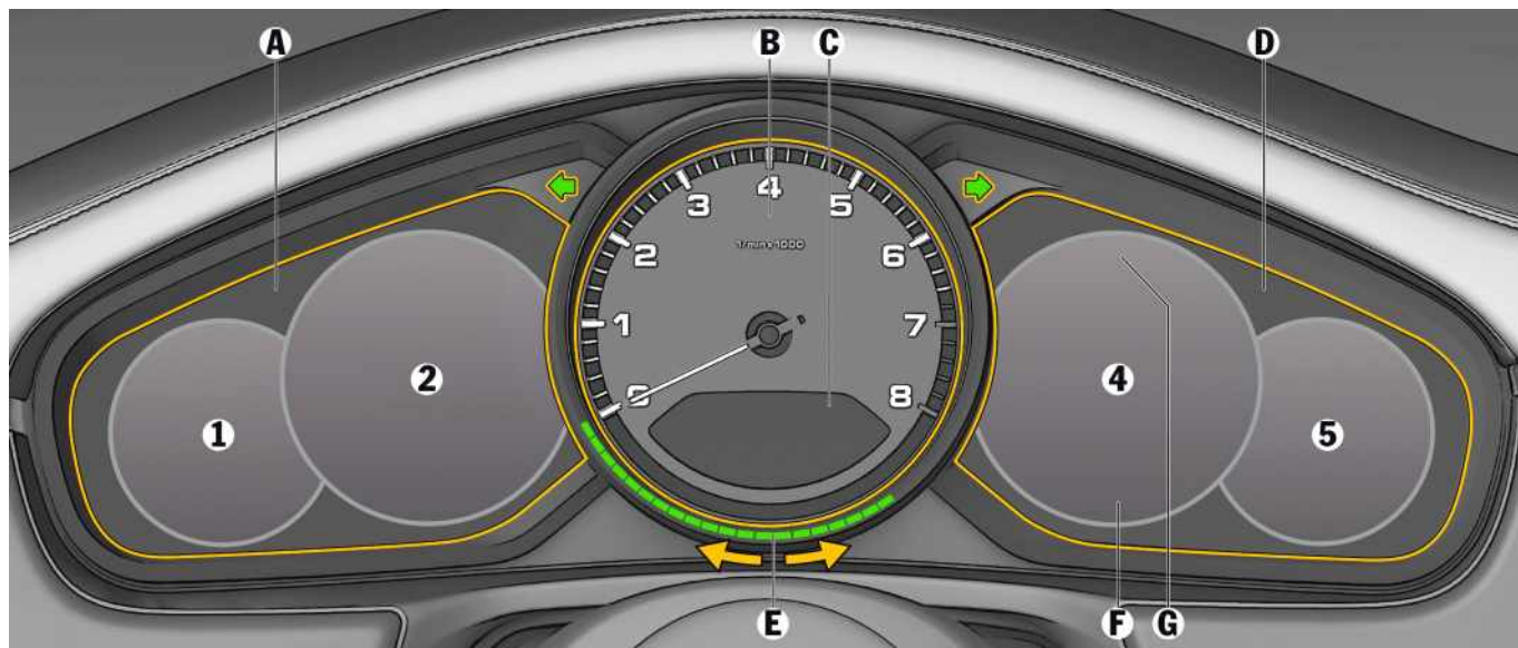
Fig. 78: Instrument cluster
