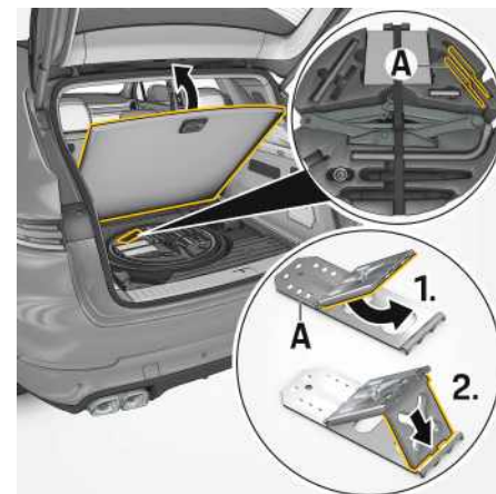
Fig. 86: Removing wedges
