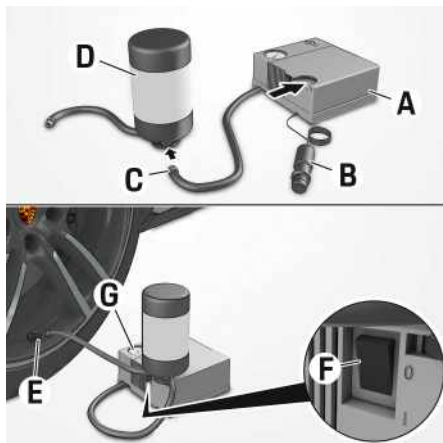
Fig. 67: Filling tire sealant
