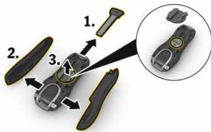
Fig. 221: Changing battery
