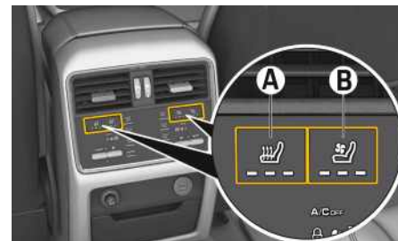
Fig. 184: Switching rear seat heating/seat ventilation on and off
