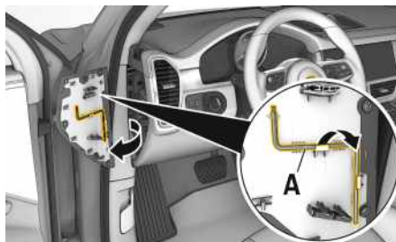
Fig. 164: Removing hexagon key
