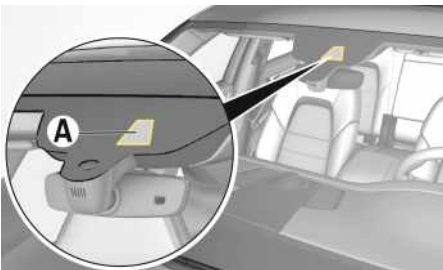
Fig. 97: Windshield camera
